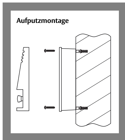
Fig. 4: Montage mural
