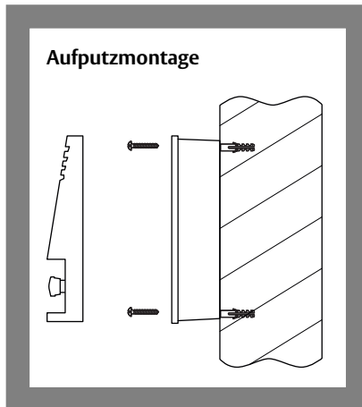
Abb. 4: Wandmontage
